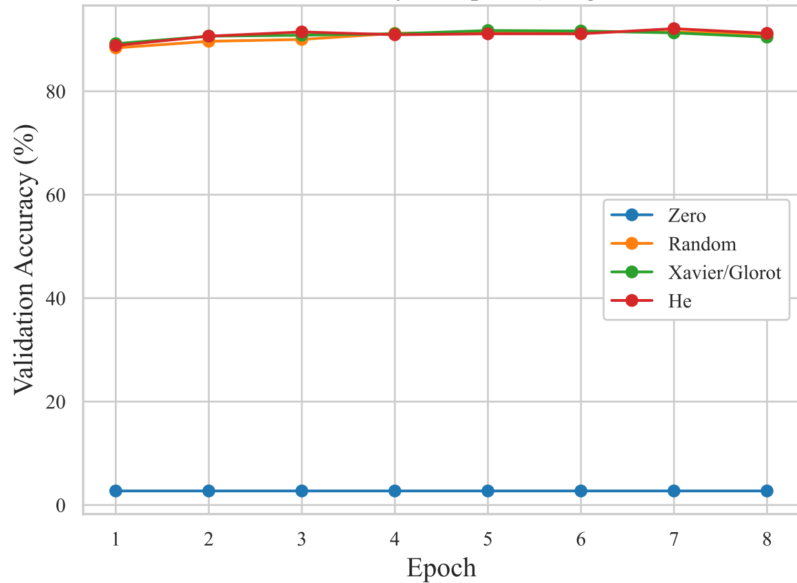
Plot 2: Validation Accuracy vs. Epoch (Weight Initialization)
